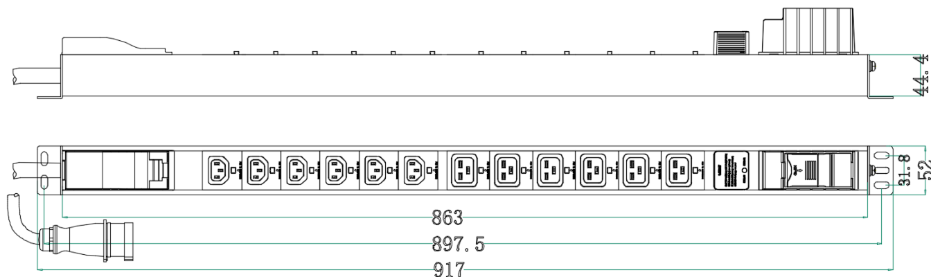
PDU Drawing
