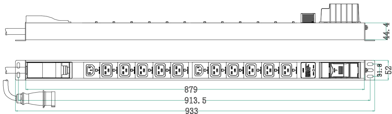
PDU Drawing
